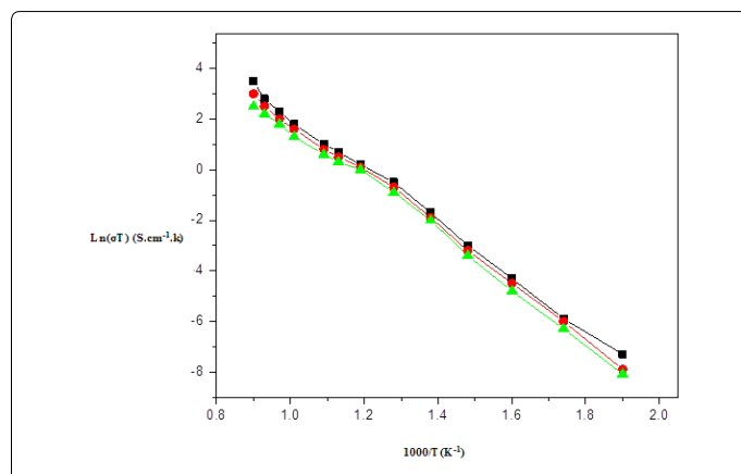
Figure 6. Arrhenius plots for the Gd_{1-x}Sr_xAlO_3 samples sintered at different ratios
