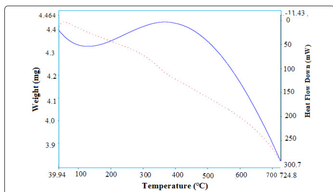
Figure 4. TGA & DTA of Gd_{0.7}Sr_{0.3}AlO_3
