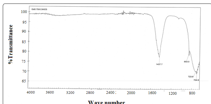
Figure 5. FT-IR spectrum of Gd_{0.7}Sr_{0.3}AlO_3
