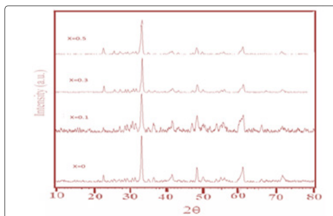
Figure 2. X-ray diffraction pattern of Gd_{1-x}Sr_xAlO_3
