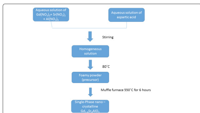
Figure 1. Flow chart of assisted combustion synthesis of Gd_{1-x}Sr_xAlO_3
