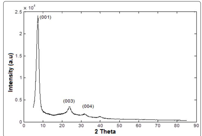
Figure 4. XRD pattern for the deposited vanadium pentoxide film on glass substrate (d=927 nm).
