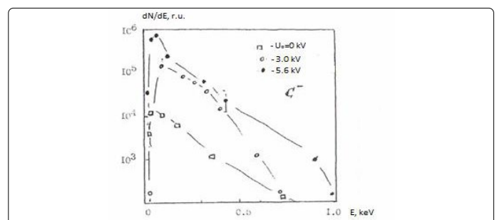
Figure 22. Dependence of the electrode potential on the energy distribution of the negative carbon ions.
