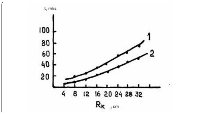
Figure 33. Dependences of the atom flux durations on the ring radius R_{\text{ring}} at (1) 2.5 \times 10^8 and (2) 4.3 \times 10^8 \text{ W/cm}^2 .
