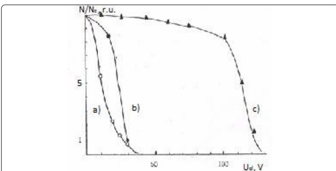
Figure 10. Relative number of electrons as a function of different distances between the electrode and the target [(a) 55, (b) 85, and (c) 8mm].
