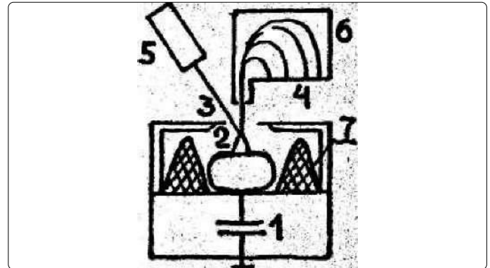
Figure 25. Experimental setup for studying the 'fast' LF: (1) capacitor, (2) and (3) electrodes, (4) film, (5) laser, (6) analyzer, (7) insulator.
