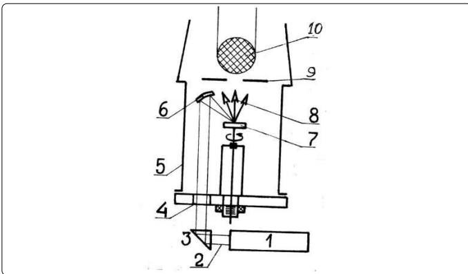
Figure 29. Arrangement of the peripheral source.
