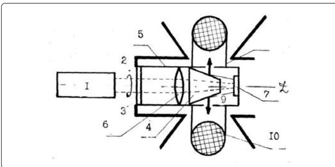
Figure 37. Scheme of the central version of the laser source CHIA in the adgesator chamber.
