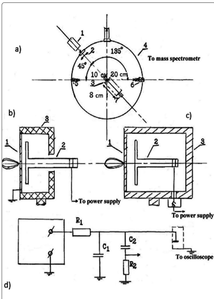
Figure 1 (a,b,c,d). (a) Schematic of the experimental setup: (1) LTI PCh-8 laser, (2) focusing lens, (3) target, (4) interaction chamber, (5, 6, 7) electrodes. (b) Target unit design with an open electrode: (1) target, (2) electrode, (3) housing. (c) Target unit design with an isolated electrode: (1) target, (2) electrode, (3) housing. (d) Scheme of electrode connection to the power supply.
