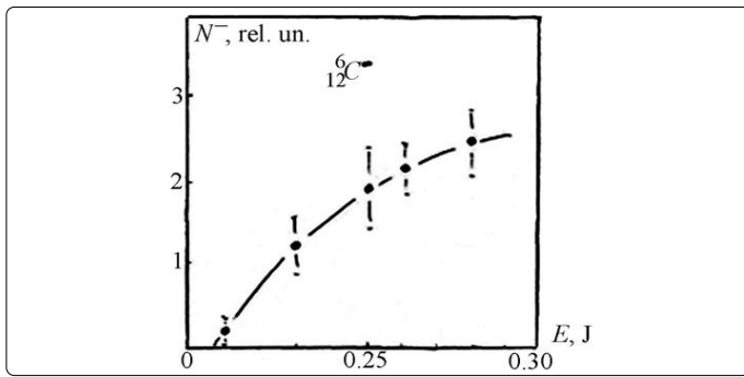
Figure 23. Dependence of the number of negative carbon ions on the additional inputted energy in the case of LF pinching.
