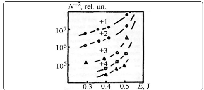
Figure 21. Dependence of the number of aluminum ions on the energy inputted into the LF.
