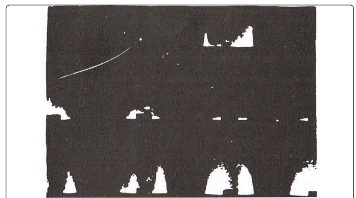
Figure 18. LF development taken by the high-speed camera (frame exposure, 500ns; voltage, 29kV; pressure, 10Pa; target, polyethylene).
