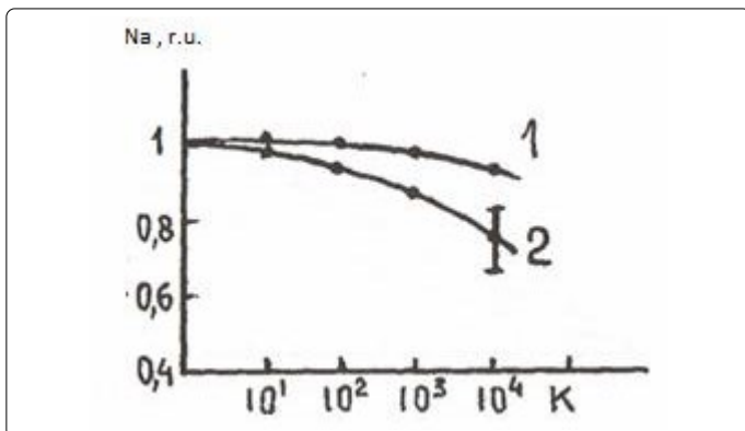
Figure 35. Dependences of the concentration of (1) iron and (2) lead atoms on the number of laser shots.
