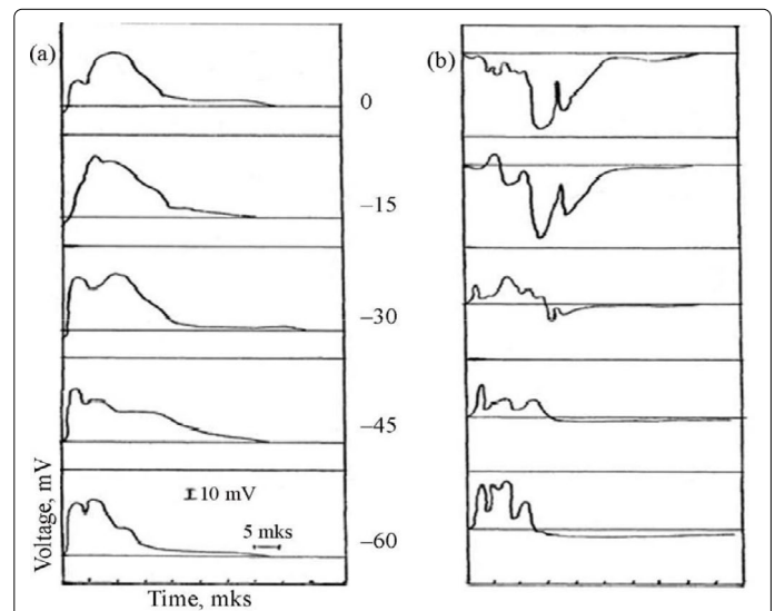
Figure 11. Oscillograms of (a) ion and (b) electron signal for a ring electrode at U_{el} = (from top to bottom) 0, -15, -30, -45, and -60 V.
