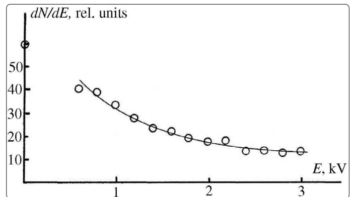
Figure 2. Dependence of the number of singly charged copper ions on the voltage applied to the electrode (for the ion energy E = 180 eV).
