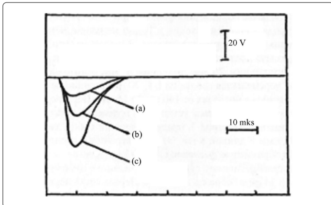
Figure 4. Typical oscillograms of the current pulses in the electrode circuit [(a) U=0 V, (b) U=100 V, and (c) U=150 V].
