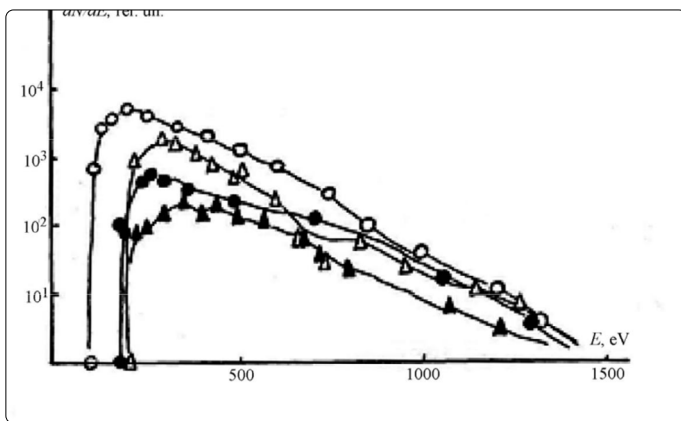
Figure 5. Energy distributions of copper ions [(○) Z=1 , (△) Z=2 at U=3 kV (open circles), and (●) Z=1 , (▲) Z=2 at U=1 kV and C=4\mu F (filled circles)].
