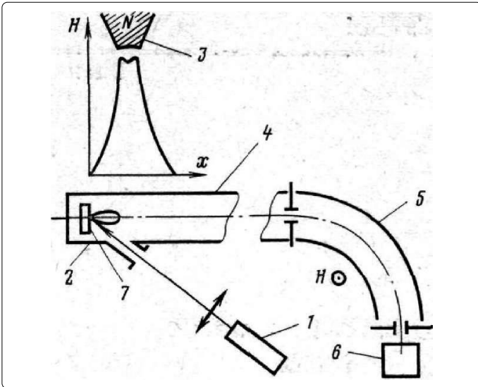
Figure 13. Scheme of the experimental setup: (1) laser, (2) vacuum chamber, (3) electromagnet pole, (4) time-of-flight tube, (5) magnetic energy analyzer; (6) SEM, (7) target.
