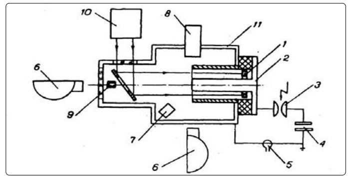
Figure 17. Scheme of the PF setup and location of the diagnostic equipment: (7) target, (2) injector, (3) discharge gap, (4) capacitor bank, (5) Rogowski coil, (6) SFR-2M photographic recorder, (7) pinhole camera, (8) thermoluminescent sensor, (9) Faraday cup, (10) CO 2 laser, (11) vacuum chamber.
