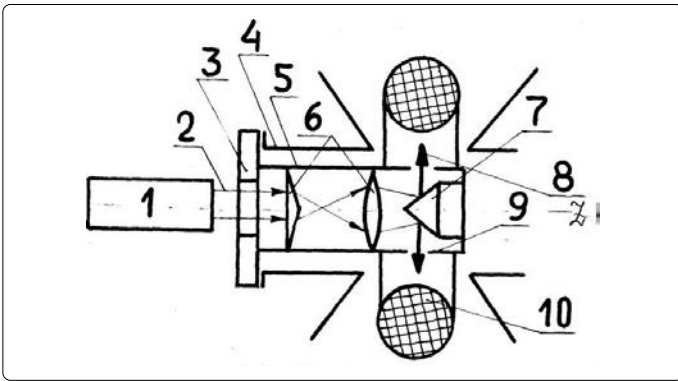
Figure 36. Scheme of the modified version of the central atom source.
