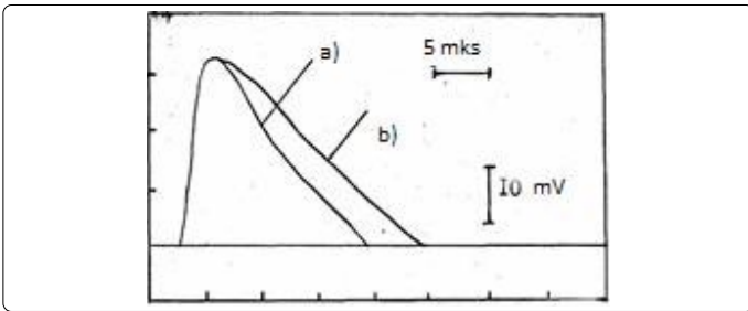
Figure 8. Oscillograms of the ion current under the action of the electric field at different target distances between the electrode and the target [(a) 55 mm, (b) 85 mm].
