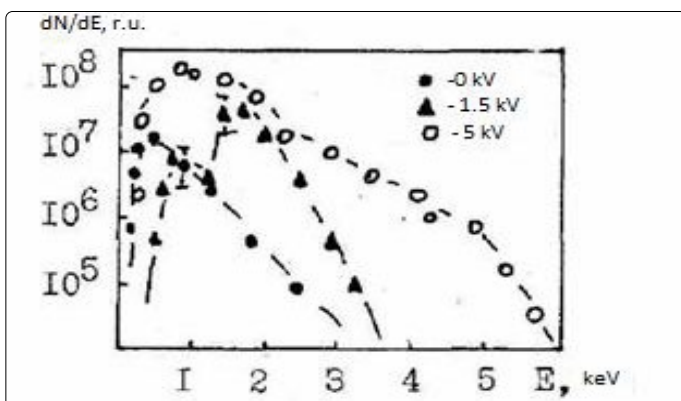
Figure 20. Energy distributions of aluminum as a function of the voltage at the capacitor V_0 .
