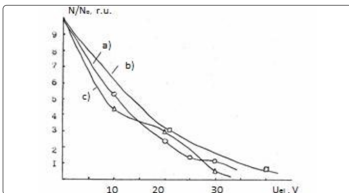
Figure 12. Relative number of electrons as a function of the electric field of a)-(○) molybdenum, b)-(□) copper, and c)-(Δ) carbon.
