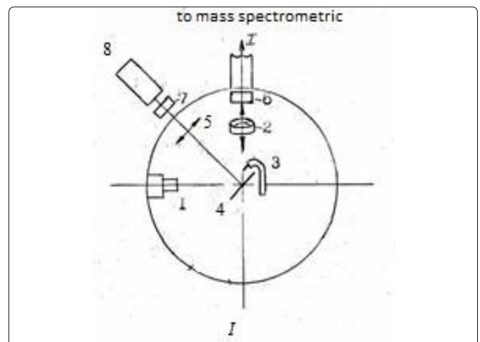
Figure 7. Scheme of the electrode arrangement: (1, 2, 3) electrodes, (4) target, (5) focusing lens, (6) ion collector, (7) filter, (8) LTI-5 laser.
