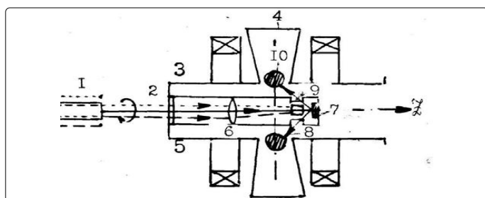
Figure 27. Scheme for loading a compressed electron ring (central version of a source of atoms).
