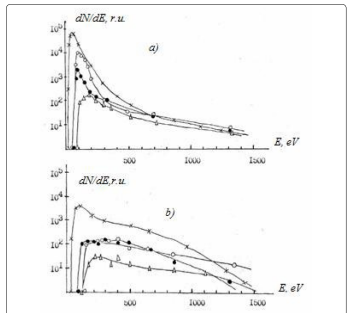
Figure 6. Change in the energy distributions of molybdenum ions [(a) Z=1 , (b) Z=2 ; (○) electrode (7) and U=500 V; (●) electrode (6) and U=1 kV; (▲) electrode (5) and U=100 ; (x) U=0 ].
