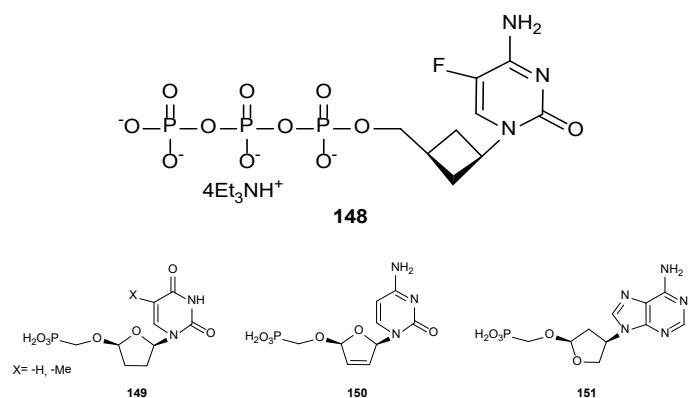
Scheme 43. Nucleoside analogues (148-151).
