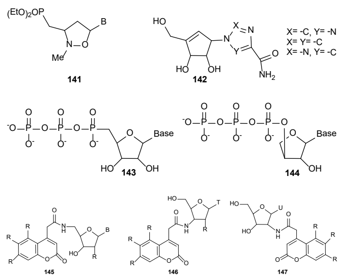
Scheme 42. Ribose derivatives (141-147)
