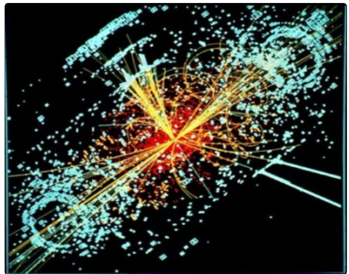
Figure 1. Higgs field and mass to the elementary particles
